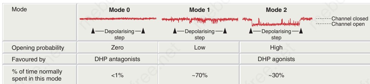
Fig. 22.12 Mode behaviour of calcium channels. The traces are patch clamp recordings (see Ch. 3) of the opening of single calcium channels ( downward deflections ) in a patch of membrane from a cardiac muscle cell. A depolarising step is imposed close to the start of each trace, causing an increase in the opening probability of the channel. When the channel is in mode 1 ( centre ), this causes a few brief openings to occur; in mode 2 ( right ), the channel stays open for most of the time during the depolarising step; in mode 0 ( left ), it fails to open at all. Under normal conditions, in the absence of drug, the channel spends most of its time in modes 1 and 2, and only rarely enters mode 0. DHP, dihydropyridine. (Redrawn from Hess, et al., 1984. Nature 311, 538–544.)
