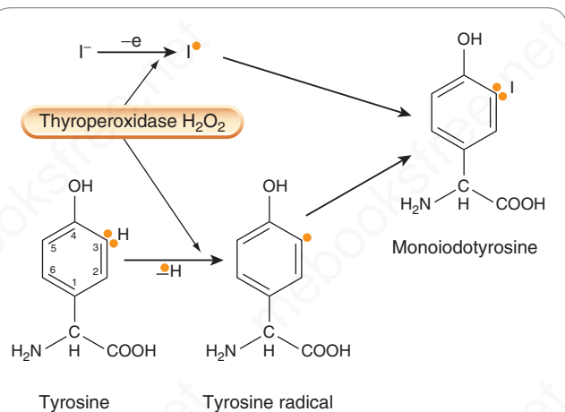
Fig. 35.2 Iodination of tyrosyl residues by the thyroperoxidase- \text{H}_2\text{O}_2 complex. This probably involves two sites on the enzyme, one of which removes an electron from iodide to give the free radical \text{I}\cdot ; another removes an electron from tyrosine to give the tyrosyl radical (shown by orange dot). Monoiodotyrosine results from the addition of the two radicals.
